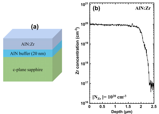
FIG. 1. (a) Schematic layer structure of AlN:Zr produced by MOCVD. (b) Plot of the Zr concentration profile measured by SIMS, revealing a uniform Zr concentration of 10^{20} \text{ cm}^{-3} along the c-axis in the entire AlN:Zr epilayer.
